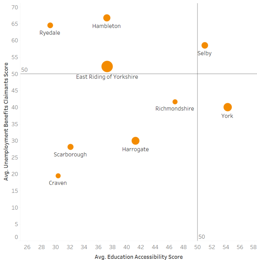
Average of Unemployment Benefits Claimants Score vs Average of Education Accessibility Score for each LAD for 2021, where size shows total population of the LAD
